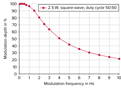
Modulation depth
