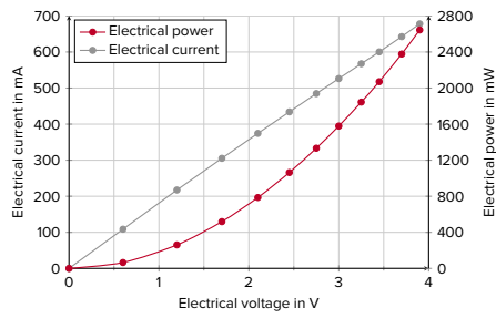
Electrical specifications
