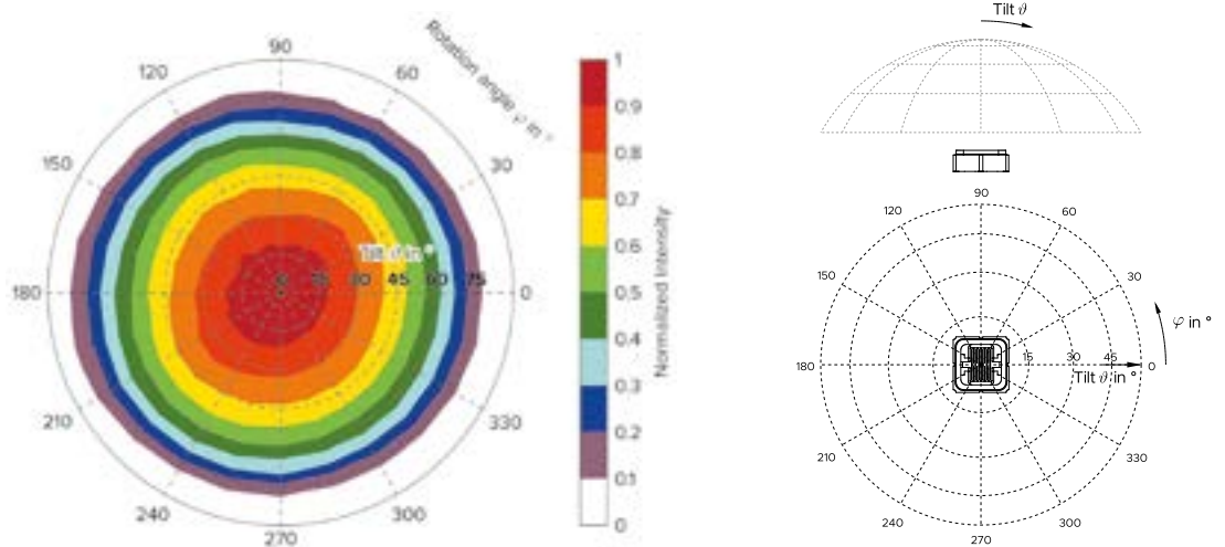
Angular radiation distribution (without window)
