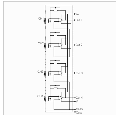
Circuit Diagram
