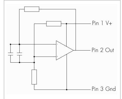
Circuit Diagram
